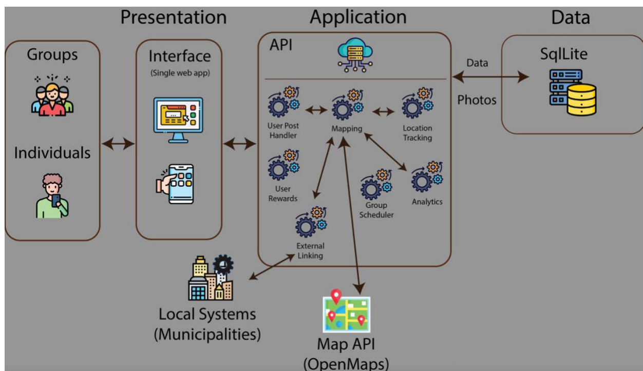
Product TrashTag Major Functional Component Diagram
